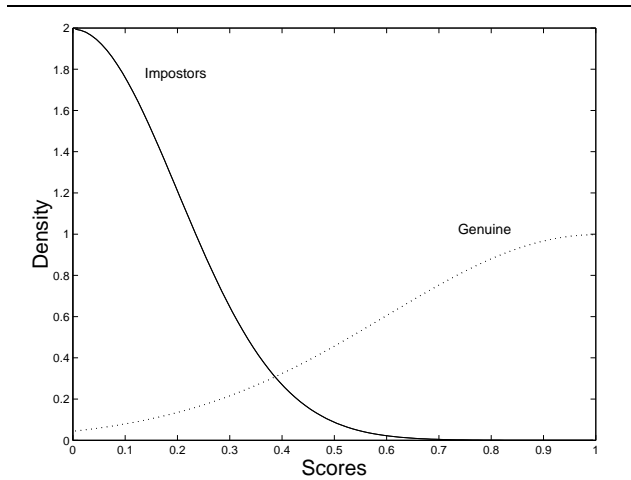
Figure 1. Chosen densities of matching(genuine) and non-matching(impostors) scores.
