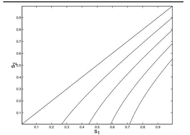
Figure 2. Bayes decision boundaries for N=2 with contours drawn for L=1,10,100,1000 and 10000.
